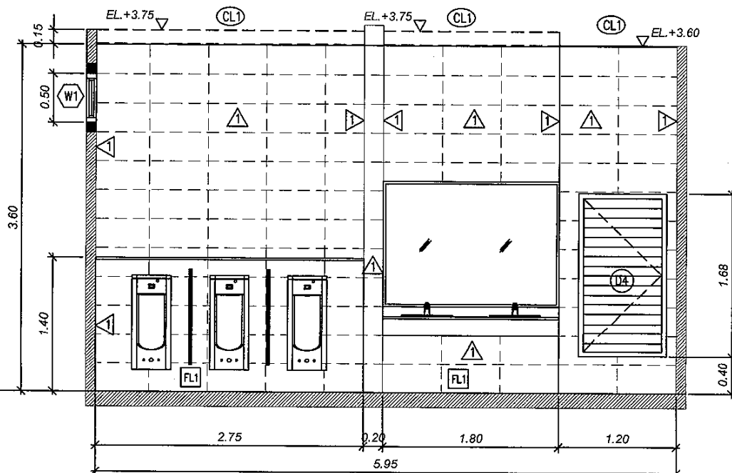
ELEVATION 2 SCALE 1:25
