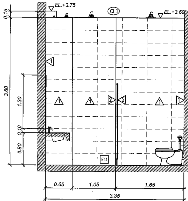
ELEVATION 1 SCALE 1:25
