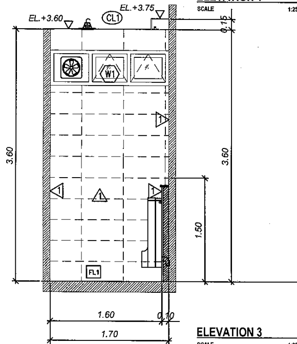
ELEVATION 1 SCALE 1:25
