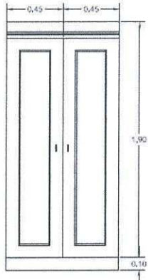
FRONT
