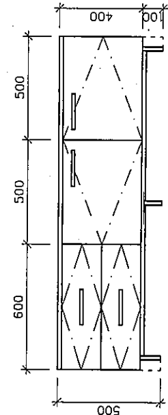
FRONT VIEW SCALE 1 : 25
