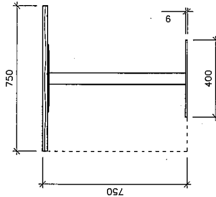
FRONT VIEW SCALE 1 : 20
