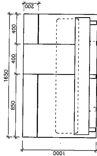
FRONT VIEW SCALE 1 : 30
