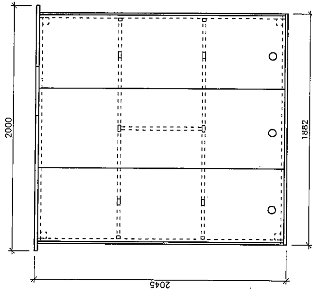
TOP VIEW SCALE 1 : 30
