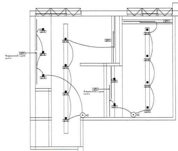
ELECTRICAL PLAN 8 st Floor
