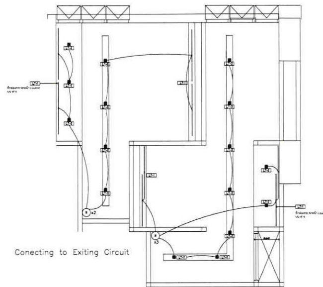
ELECTRICAL PLAN 2 st Floor
