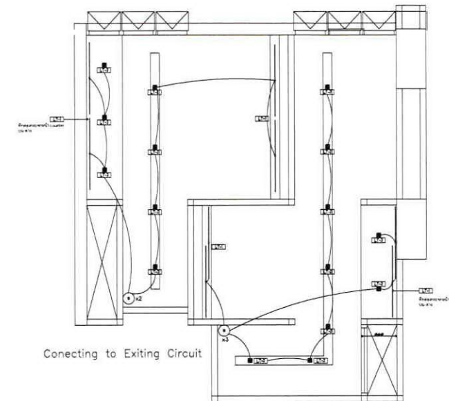
ELECTRICAL PLAN 3 st Floor
