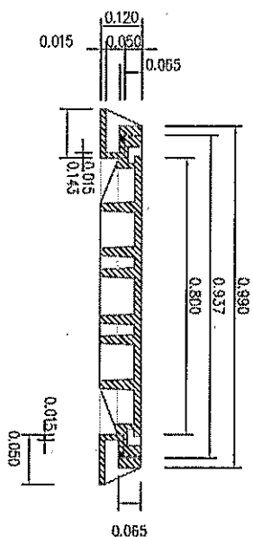
MANHOLE COVER DETAILS SCALE 1 : 10
