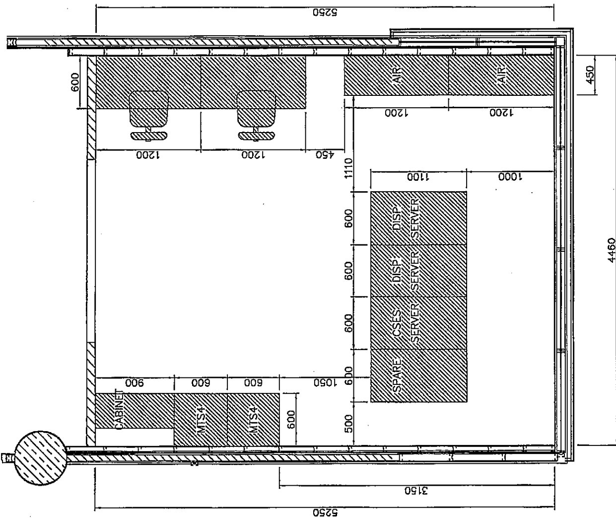
EQUIPMENT LAYOUT SCALE : 1:100
